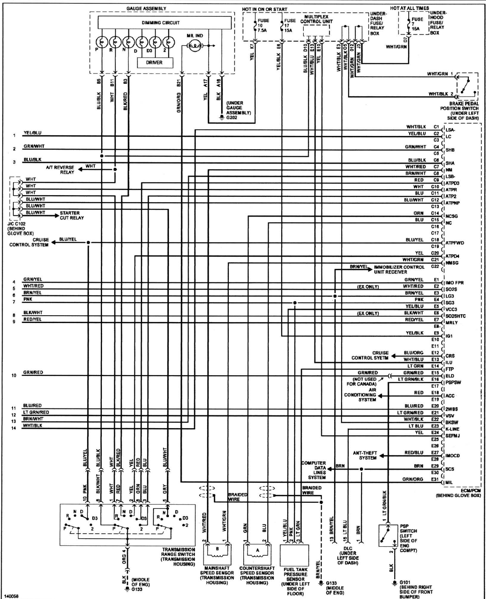
Fig. 12: Wiring Diagram (Civic Except GX & HX 1.7L - 3 Of 3)
